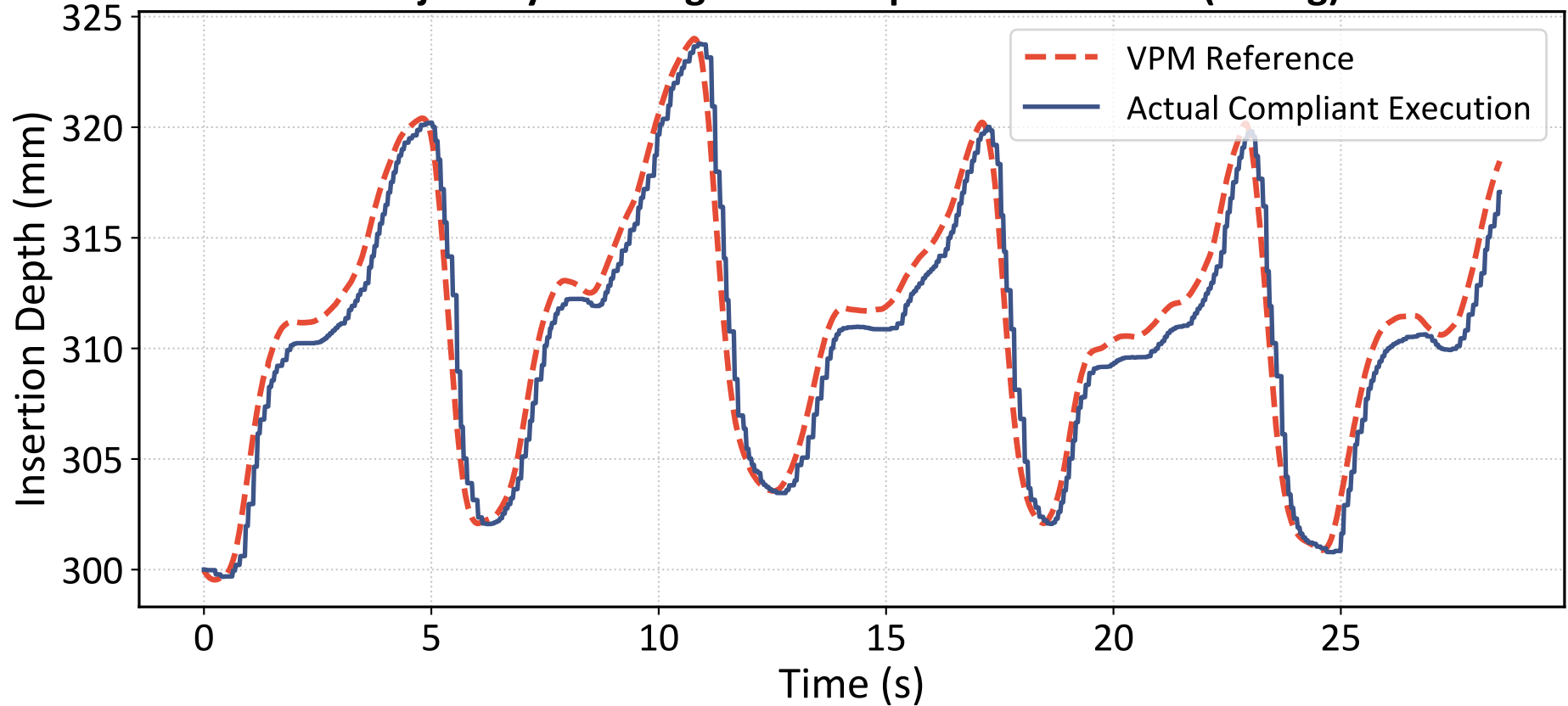
Trajectory Tracking with Compliant Retraction (Lifting)
